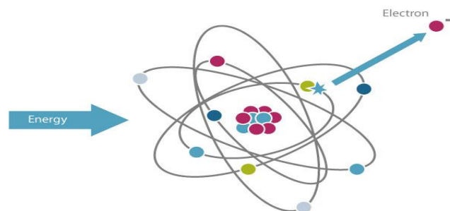
Figure 1: Knocking of electron from an atom due to exposure to ionizing radiation atom
